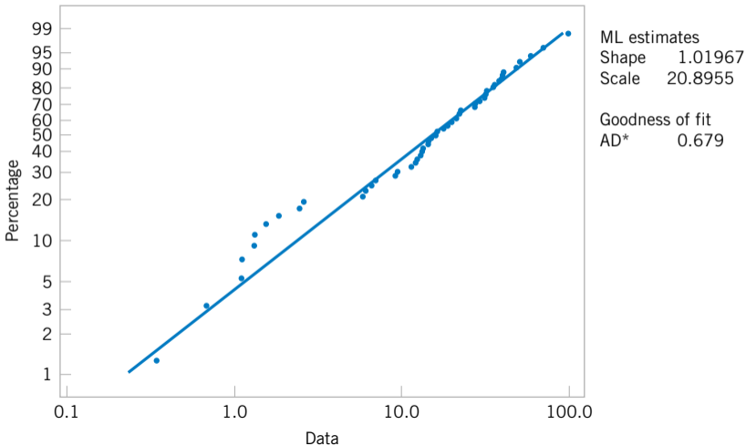
Weibull probability plot ML estimates
