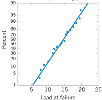
Normal probability plot
