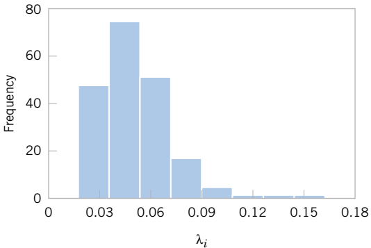
(a) Histogram of the bootstrap estimate
