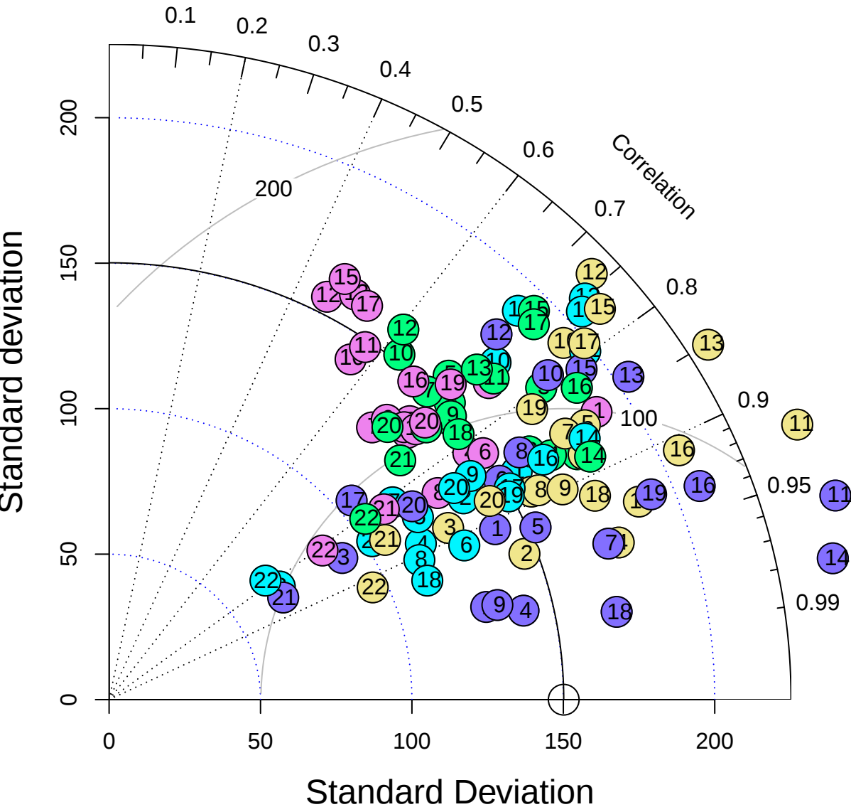
Taylor Diagram
